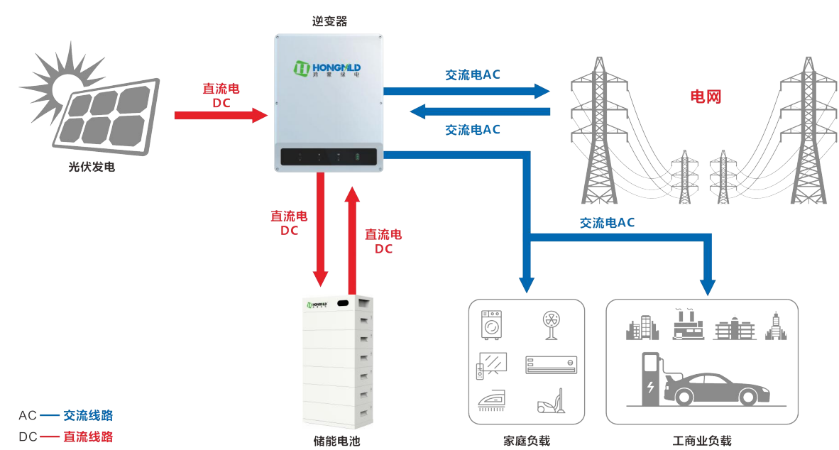
Grid-connected Schematic Diagram of PV & Energy Storage
