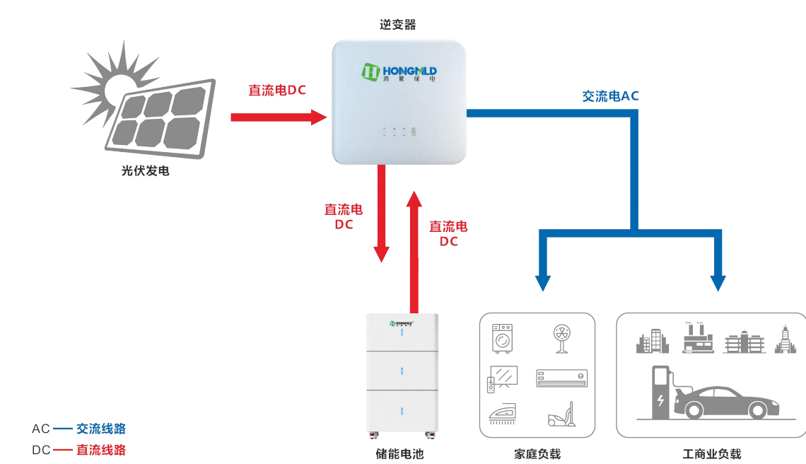
Off-grid Schematic of PV & Energy Storage
